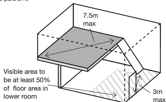
Diagram 1 Gallery floors with no alternative exit
