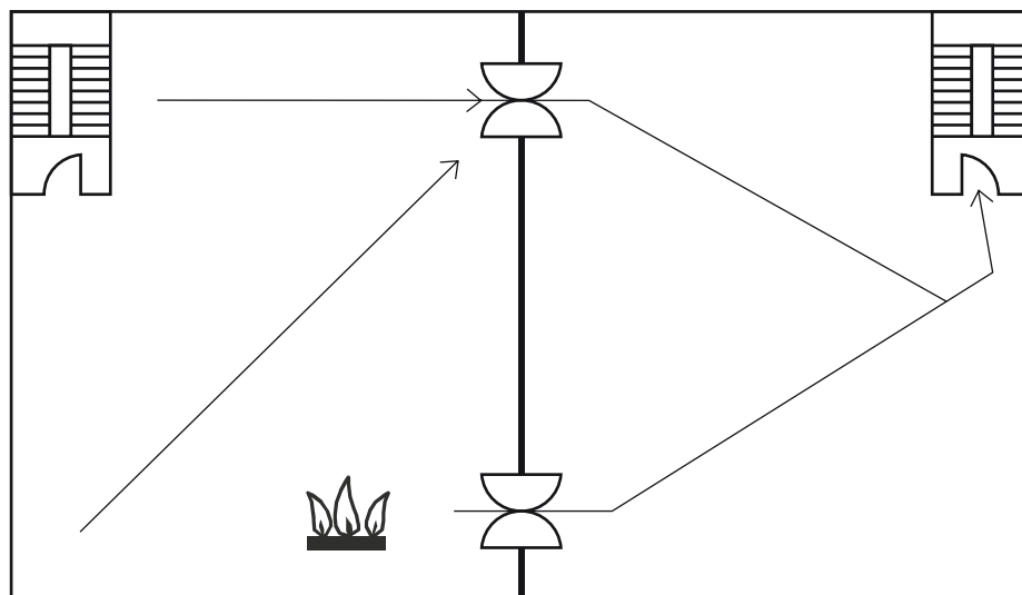
Diagram 20 Refuge formed by compartmentation
